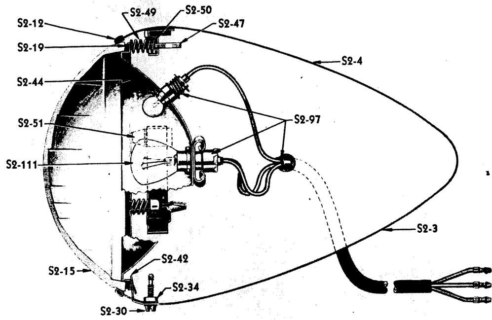
Headlamp—Hudson 112
