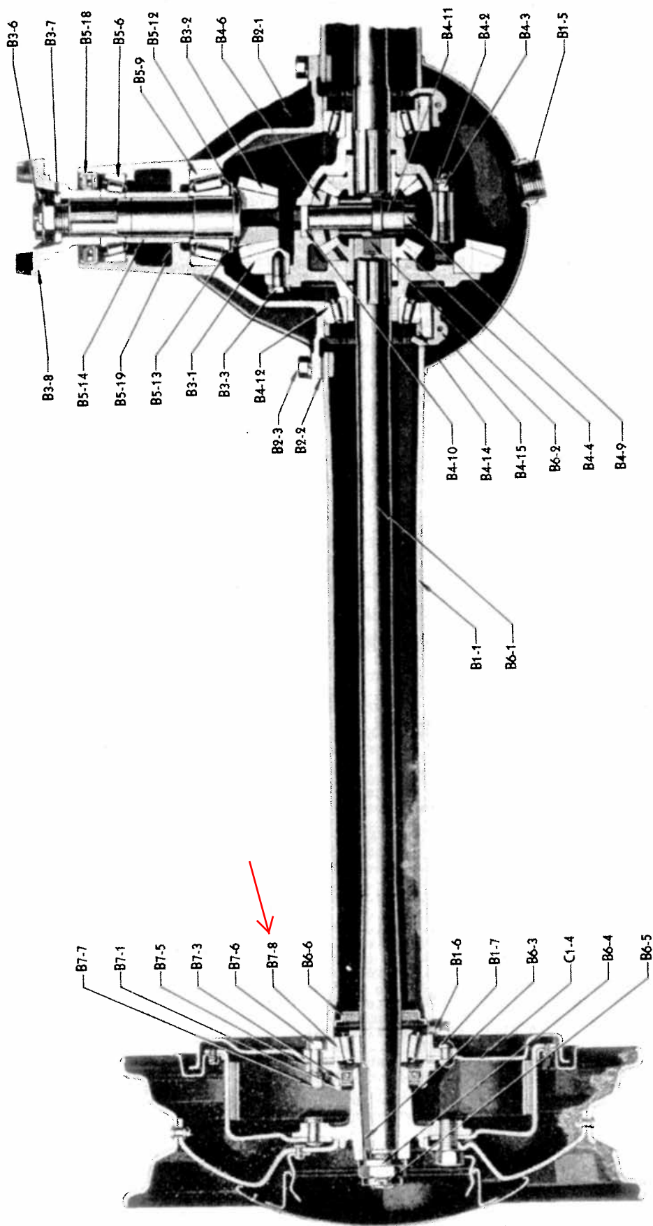
Rear Axle 1932-33 Terraplane 1934 thru 39 All Models
