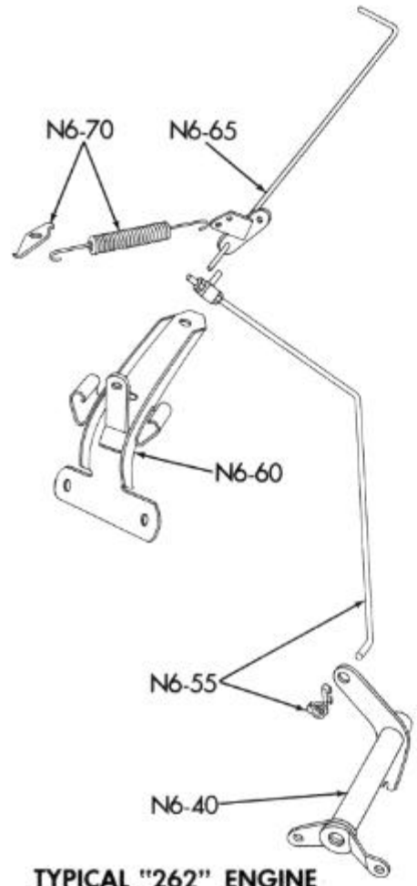
TYPICAL "262" ENGINE PACEMAKER AND WASP
